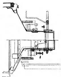
Fig. 511. Cross-Section through Player Ashpan.
